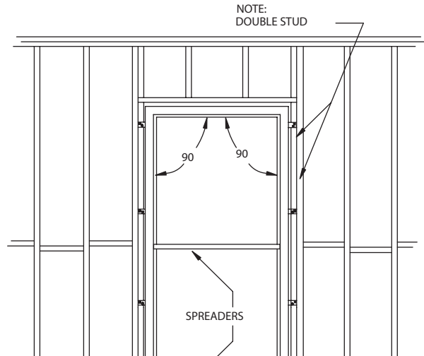
FIGURE 17A WOOD STUD WALL
