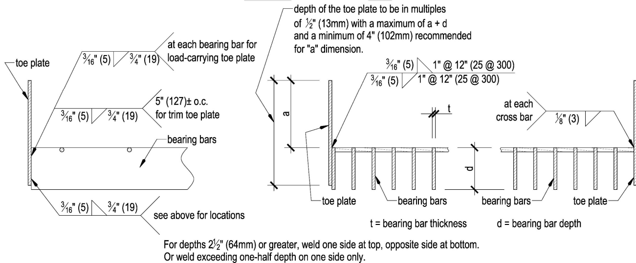
Figure 2.1.6 - TOE PLATE FOR HEAVY DUTY GRATING 2 1/2" DEEP AND GREATER (bearing bar thickness \frac{1}{8} "(6mm) and greater and bearing bar clear opening greater than or equal to \frac{5}{8} "(16mm))
