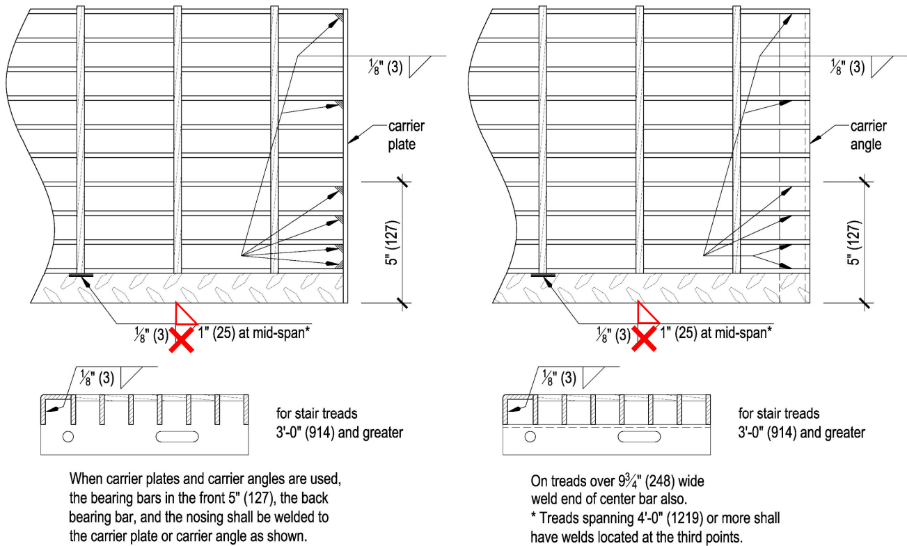
Figure 2.1.11 - STANDARD STAIR TREADS (bearing bar thickness less than 1/4" (6mm) and bearing bar clear opening greater than or equal to 5/8" (16mm))
