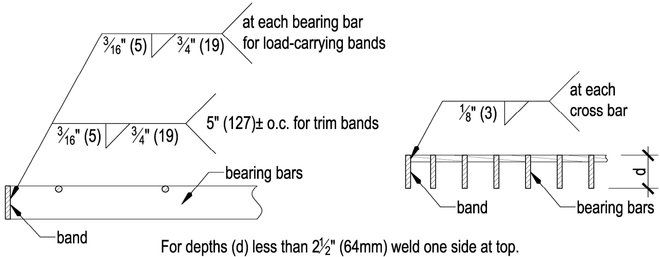
Figure 2.1.3 - BANDING FOR HEAVY DUTY GRATING LESS THAN 2 1/2" DEEP (bearing bar thickness \frac{3}{8} " (6mm) and greater and bearing bar clear opening greater than or equal to \frac{5}{8} " (16mm))
