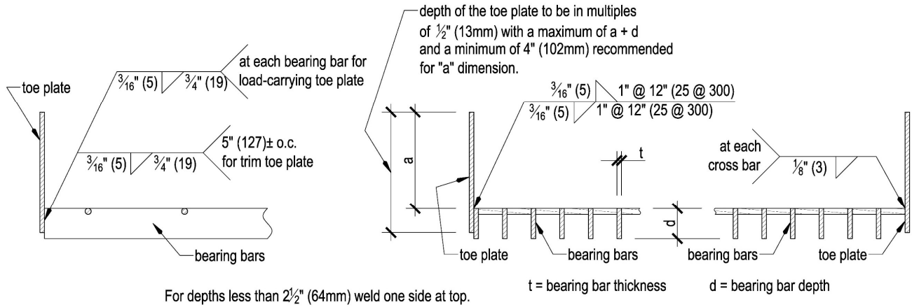
Figure 2.1.5 - TOE PLATE FOR HEAVY DUTY GRATING LESS THAN 2 1/2" DEEP (bearing bar thickness \frac{1}{8} "(6mm) and greater and bearing bar clear opening greater than or equal to \frac{5}{8} "(16mm))
