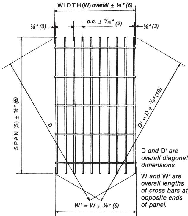
overall dimensions and squareness Sweep 1/200 of Span
