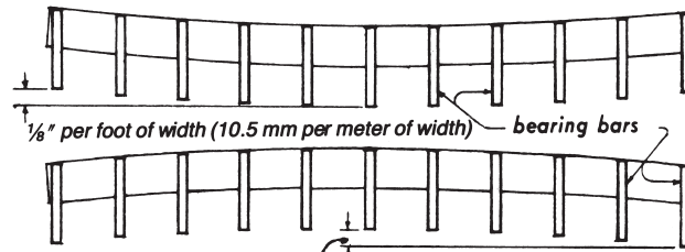
\frac{1}{8}'' per foot of width (10.5 mm per meter of width) transvers bow (before fastening to supports)
