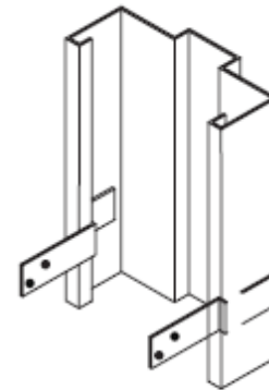
FIGURE 19C SLIP-ON DRY WALL BASE ANCHOR
