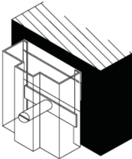
FIGURE 18B EXPANSION BOLT INSTALLATION
