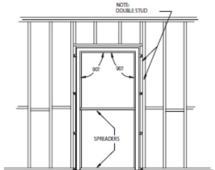
FIGURE 17A WOOD STUD WALL
