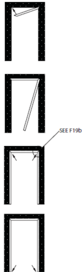
FIGURE 19A INSTALLATION SEQUENCE
