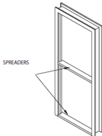
FIGURE 6 SPREADER LOCATION
