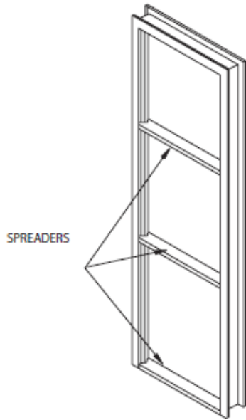
FIGURE 7 SPREADER LOCATION AT LARGE JAMB OPENING HEIGHTS
