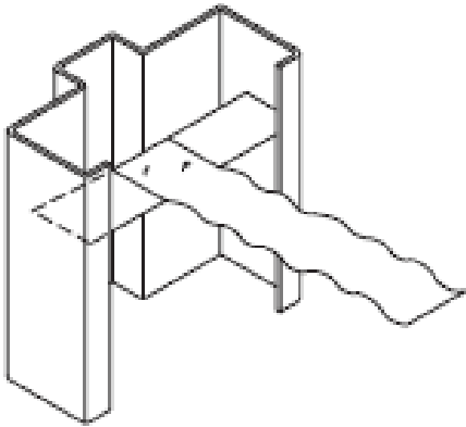
FIGURE 14C T-STRAP ANCHOR
