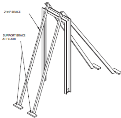
FIGURE 4 FRAME BRACING
