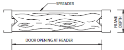
FIGURE 5 WOOD SPREADER
