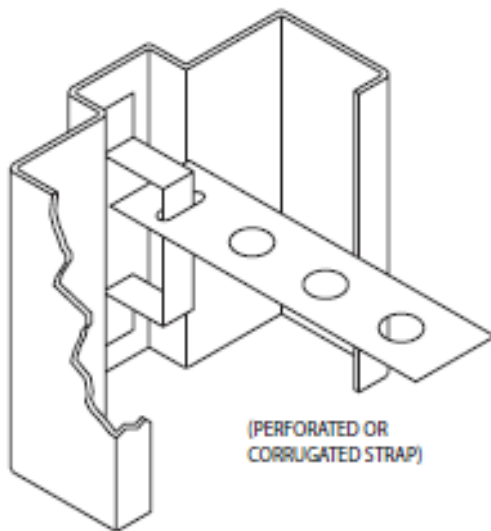
FIGURE 14B STRAP & STIRRUP ANCHOR
