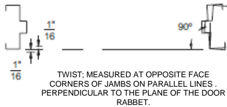
FIGURE 3 FRAME INSTALLATION TOLERANCES
