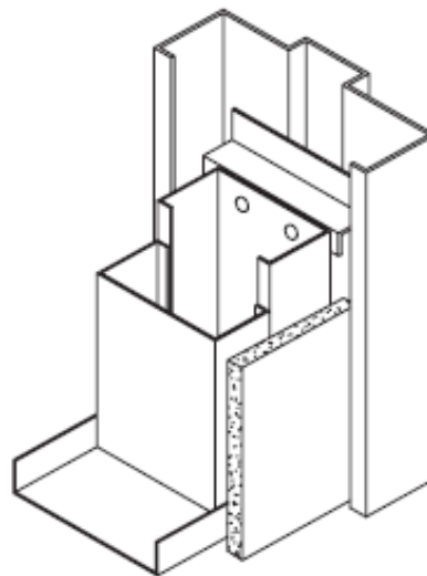
FIGURE 15C STEEL STUD WALL WITH ANCHOR
