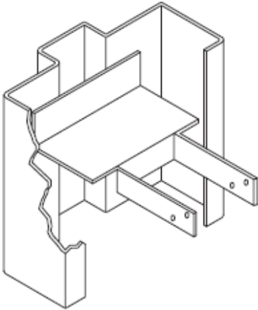
FIGURE 17D ALTERNATIVE WOOD STUD ANCHOR
