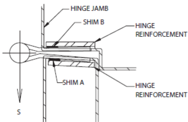
FIGURE 21 SHIMMING TO INCREASE CLEARANCE AT HINGE EDGE
