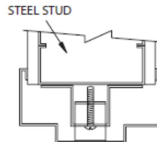
FIGURE 19D COMPRESSION ANCHORS
