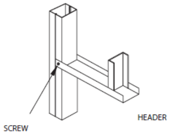
FIGURE 16D NOT RECOMMENDED
