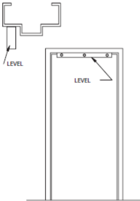
FIGURE 9 LEVELING THE HEAD
