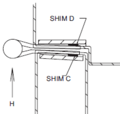
FIGURE 22 SHIMMING TO DECREASE CLEARANCE AT HINGE EDGE
