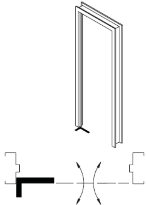
FIGURE 12 FRAME TWIST CHECK
