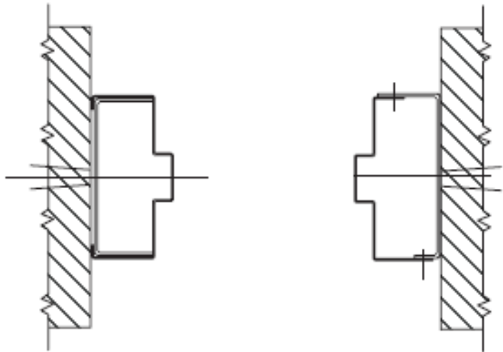
FIGURE 18C ROUGH BUCKS
